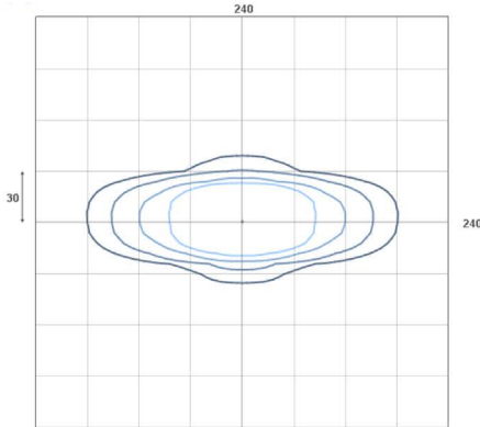
D805-LED 120W Type II
