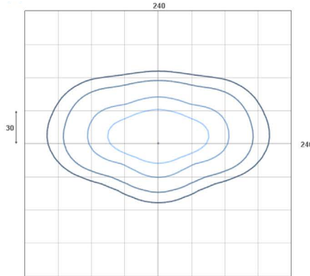
D805-LED 120W Type III/ Type IV
