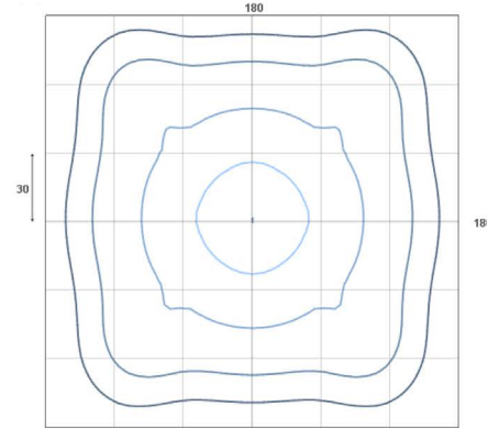
D805-LED 120W Type V
